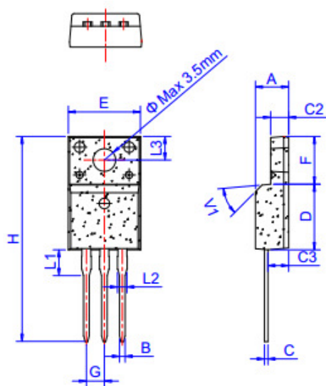
TO-220F
