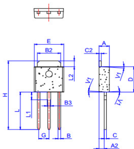
TO-220M1
