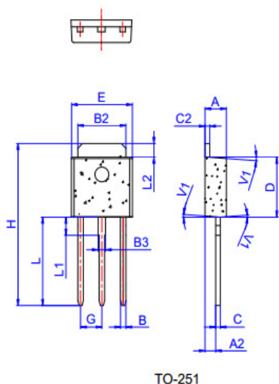
TO-251
